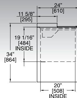
End View Flat Top Bottle Cooler 2' Model
