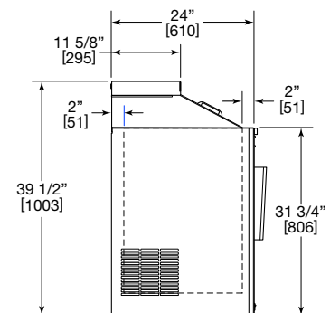
End View Slant Top Bottle Cooler For 4' & 6' Models
