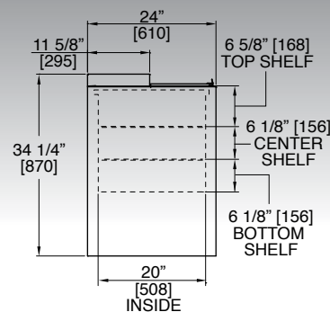
End View For 2' Model
